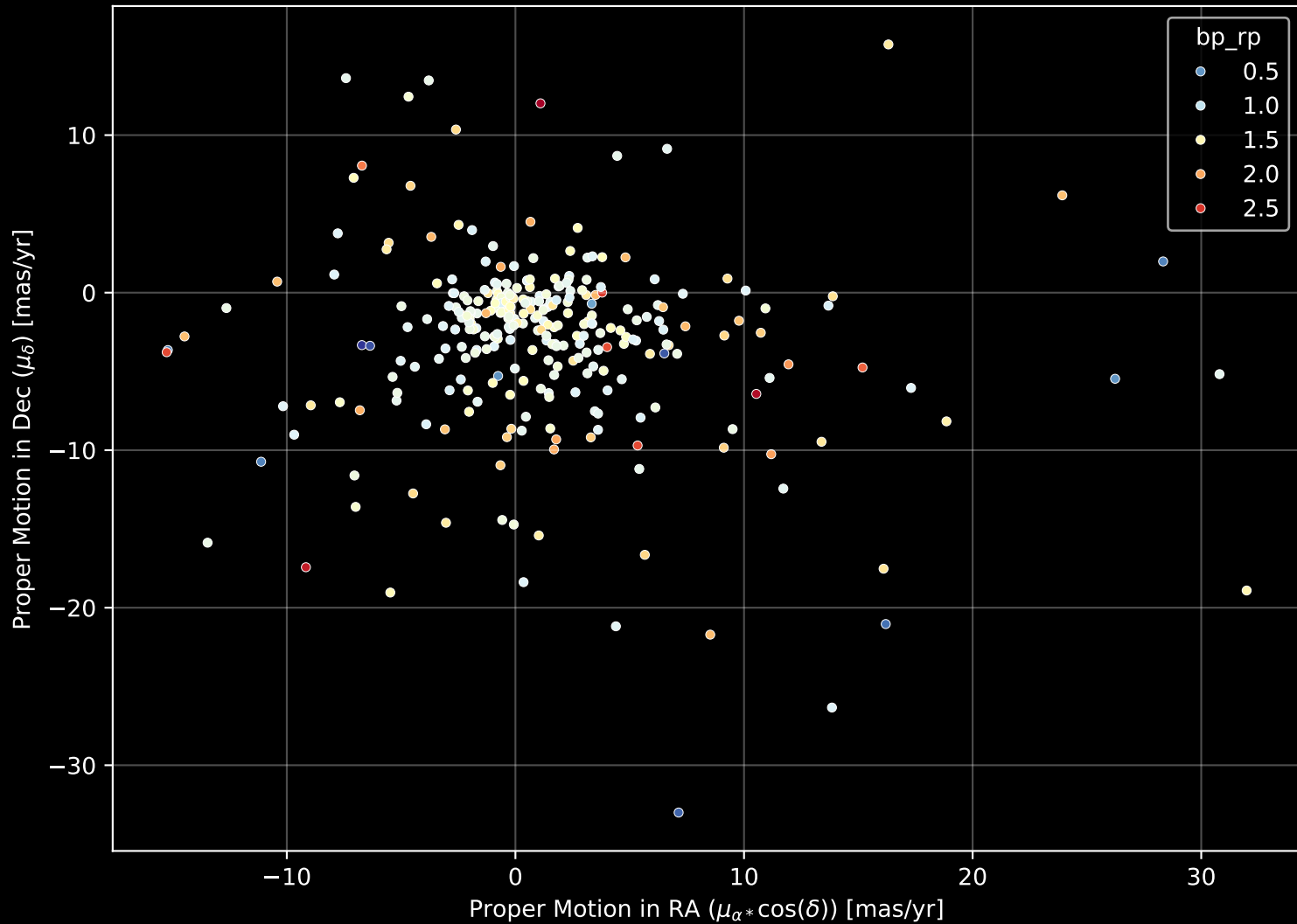
APOGEE DR17 Field: [135-24_btx] Proper Motion Diagram (n= 298)
