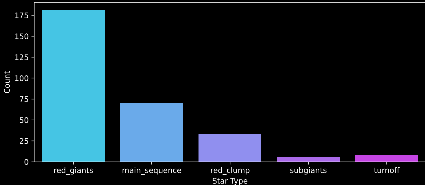
APOGEE DR17 Field: [135-24_btx] Count plot of Star Type
