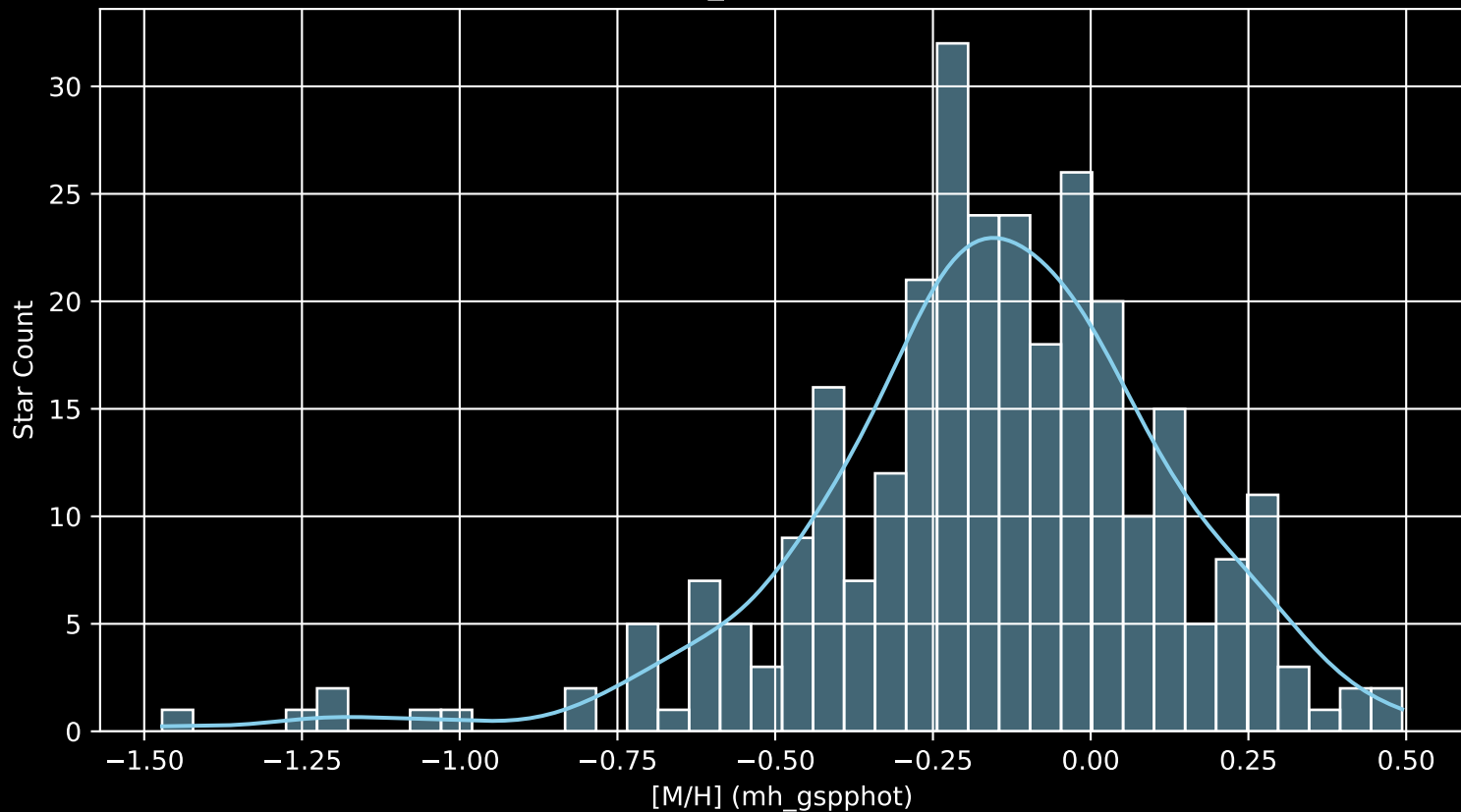
APOGEE DR17 Field: [135-24_btx [M/H] (mh_gspphot) (n= 295)
