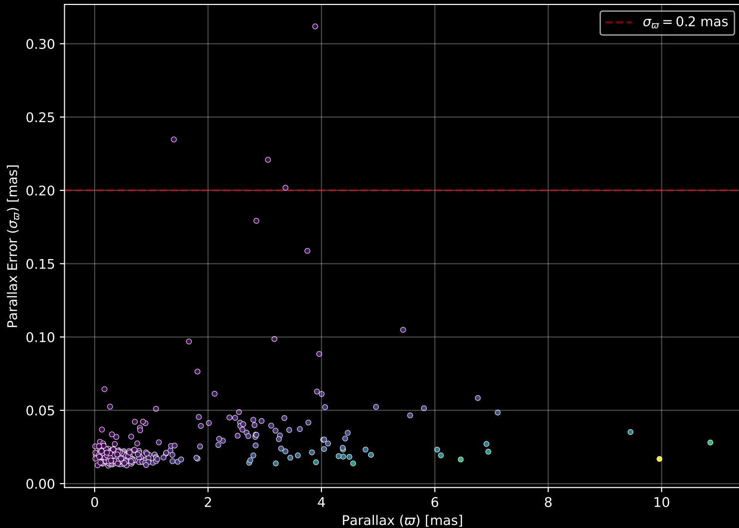
APOGEE DR17 Field: [135-24_btx] Parallax Quality (n= 298)
