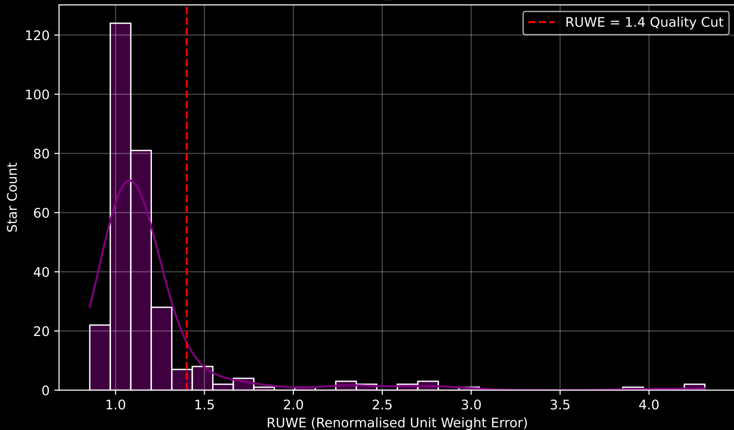
GAPOGEE DR17 Field [135-24_btx] RUWE Distribution (n= 292)
